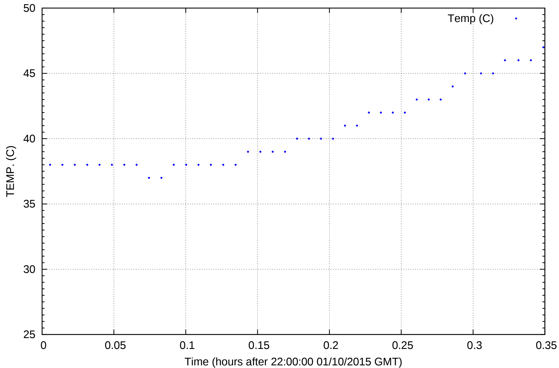
Temperature Electronics, Vacuum Pump
