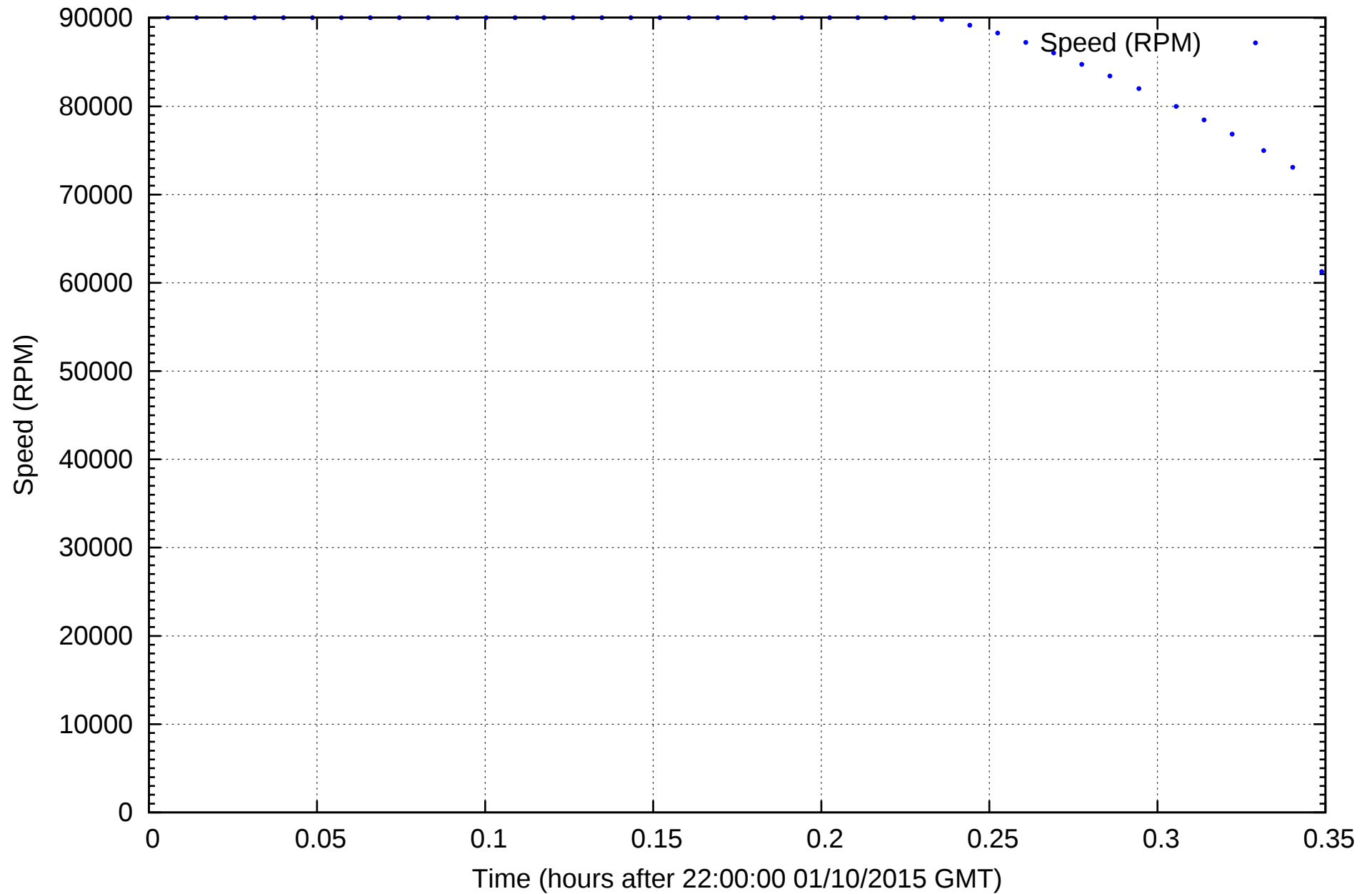
Pump Speed, Vacuum Pump
