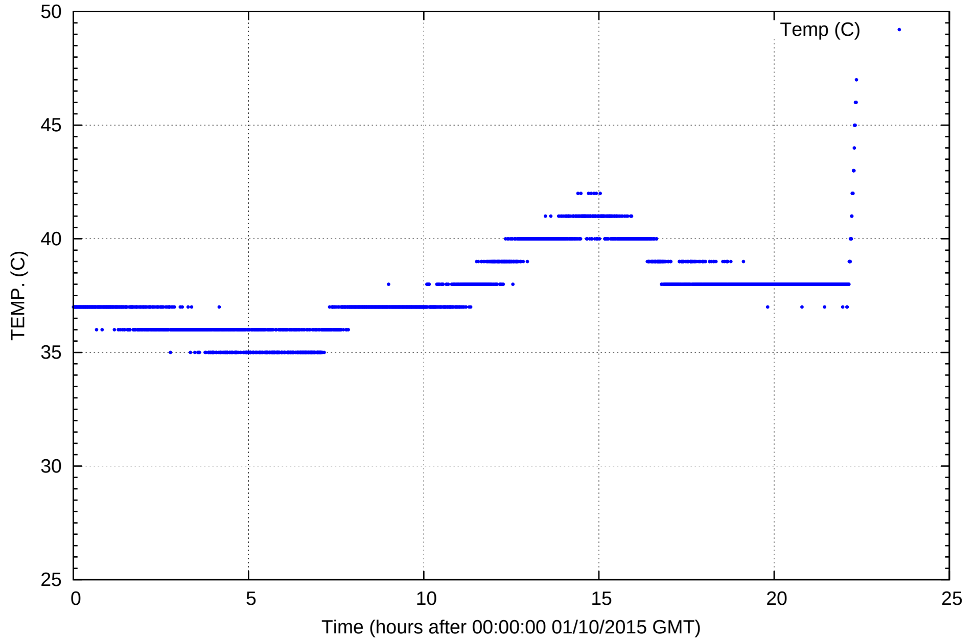
Temperature Botton, Vacuum Pump
