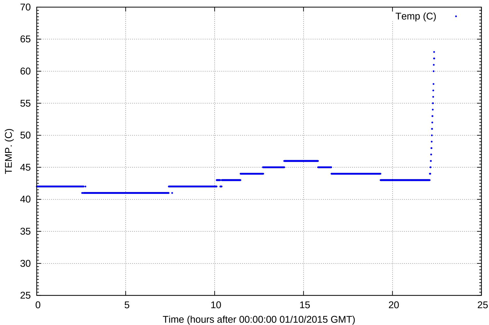
Temperature Motor, Vacuum Pump
